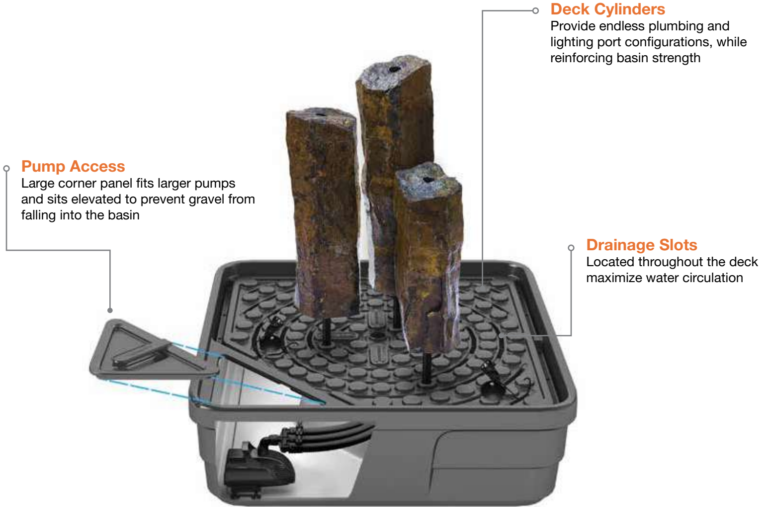
AquaBasin® 45 Shown
